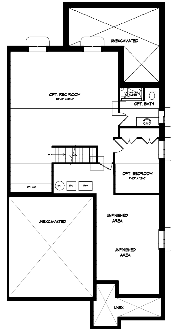
Basement
