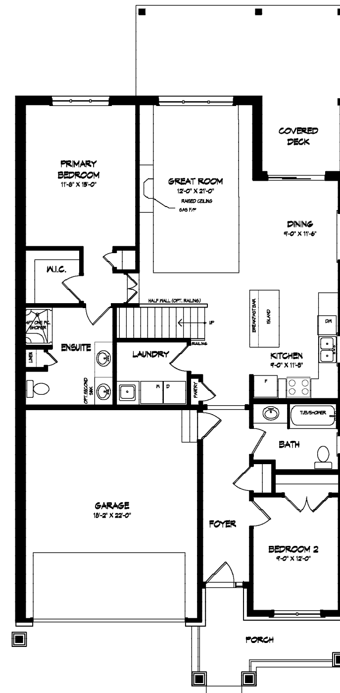
Main Floor
